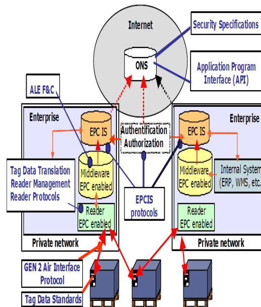
Fig 1: EPCglobal Network Standards (Source: GS1 Germany/EPCglobal)
